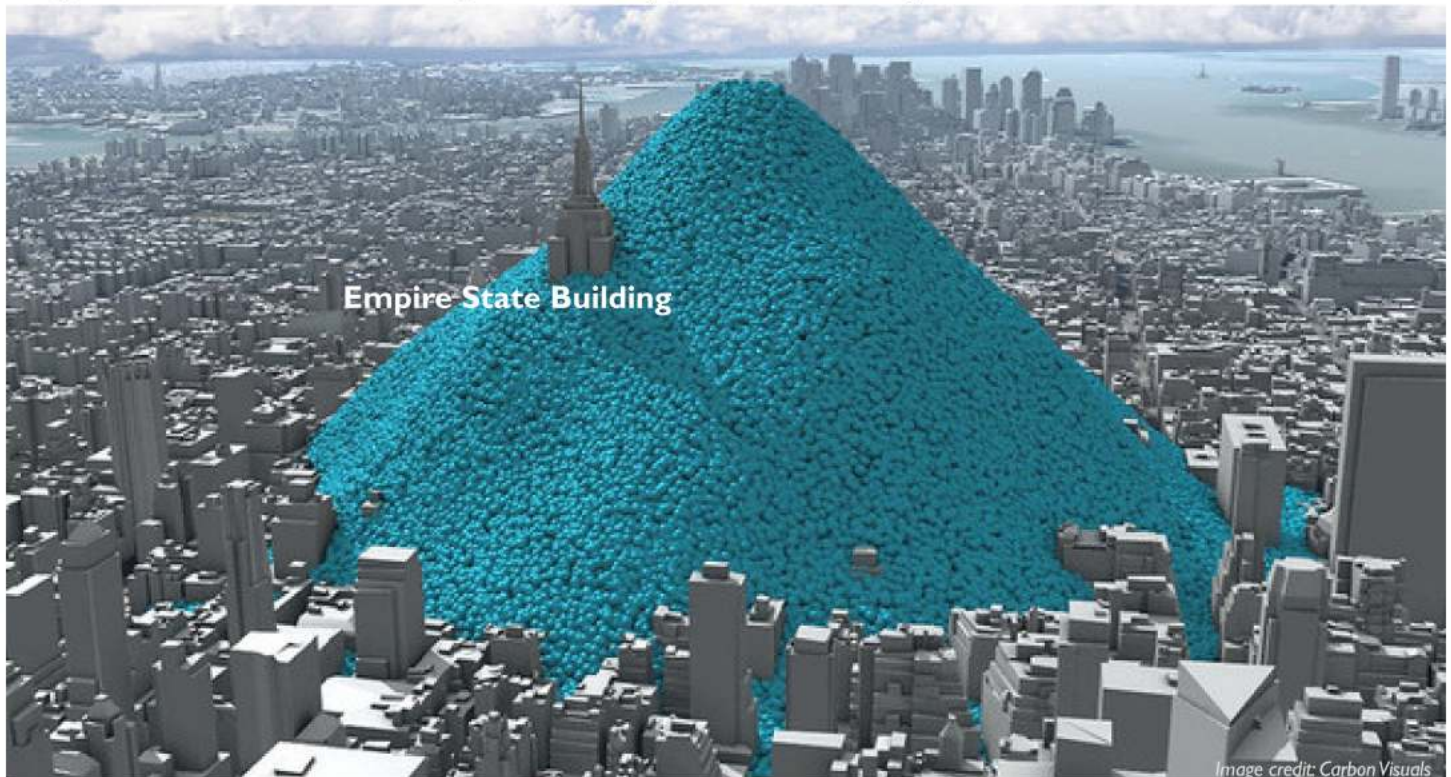
This image of New York shows one day's CO 2 production - each bubble represents one tonne of CO 2
